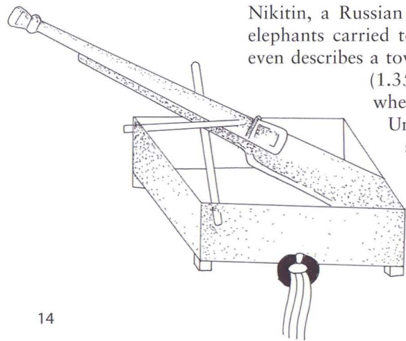
A gajnal of the time of Emperor Akbar (r. 1556–1605). The gajnal was a light cannon or large-calibre musket fastened on an elephant's back. Elephants so equipped were used in India from the early 16th to the late 17th centuries.
