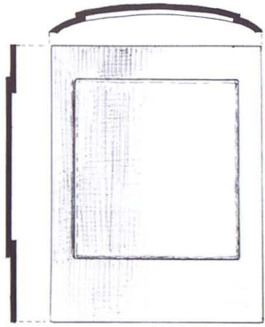
Sample of one of the 18 iron plates probably once used in elephant armour, found at Taxila and dating from the 1st century BC to 1st century AD. The plate is 25.4 x 21.6cm (10 x 8.5in). Every plate is slightly bent along its vertical axis and has a projecting central part, which was meant to enhance the protective effect: at a blow the plates spring, weakening the penetration. (After J. Marshall)
